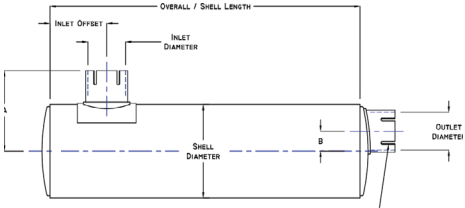
MUF4S5944
