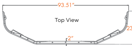
BUMGL221015 [S/P] SBFA Fog/Tow Pins/Step
